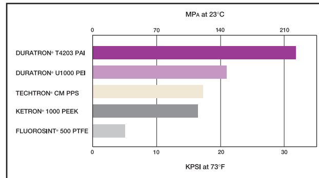
Fig. 27 - COMPRESSIVE STRENGTH COMPARISON Unfilled Grades
