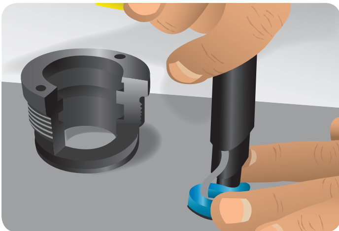
3. Pull handles back so the seal folds into itself, becoming smaller
