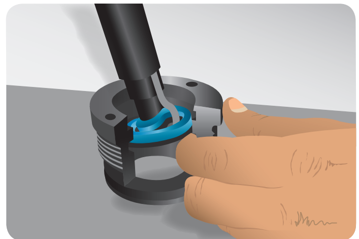
4. With a firm grip of the seal, carefully place within housing
