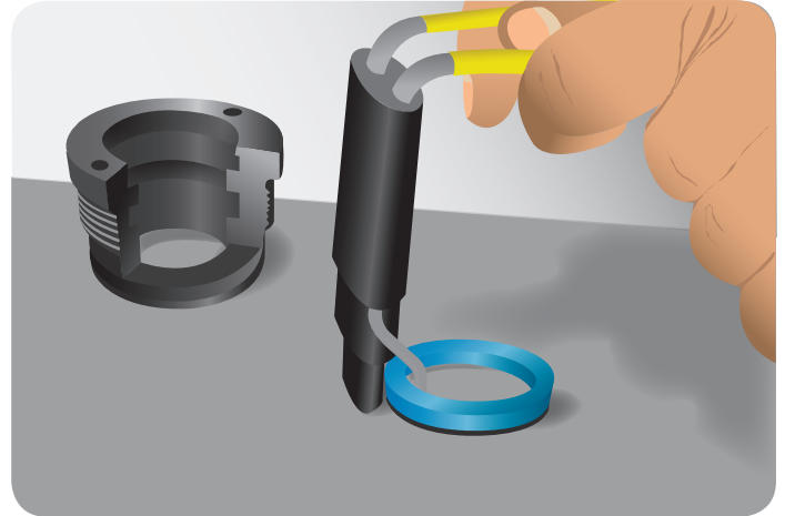
2. Place both metal tongs of installer tool inside of the seal
