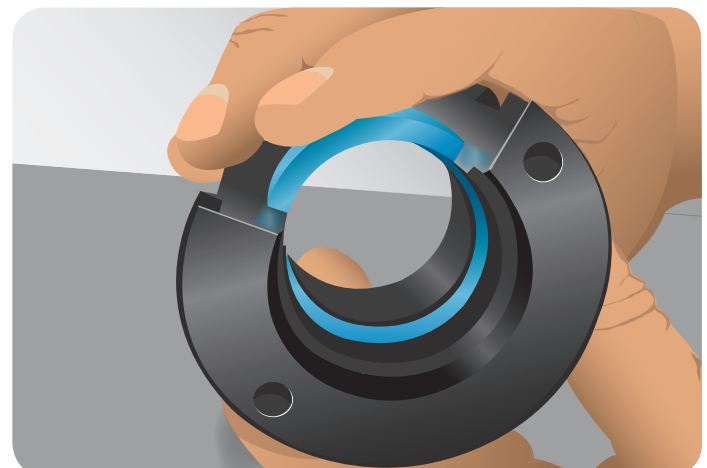
6. Once seal is properly placed inside, release grip of the installer tool
