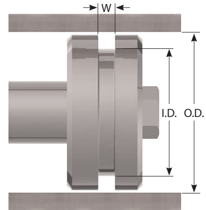
Piston Style
