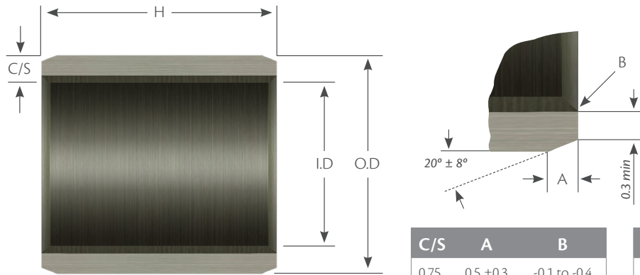
Dimensions and tolerances according to ISO 3547 and GSP Specifications
